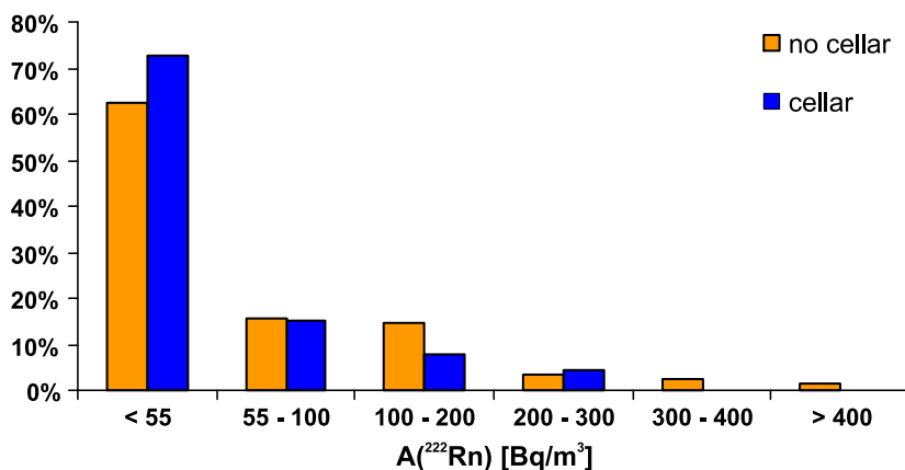
Fig. 3. The comparison of indoor ^{222}\text{Rn} concentration according to the contact of monitored room with the subsoil.
