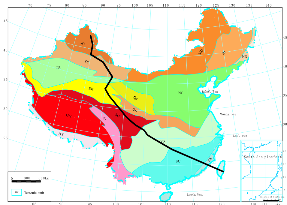
Fig. 1. Location of the transect on the schematic tectonic map (after Zhang et al. , 2011). Keys: Platforms: TR – Tarim platform, YZ – Yangtze platform, NC – North China platform; Fold systems: JG – Junggar fold system, TS – Tianshan fold system, EK – East Kunlun fold system, QI – Qilian fold system, SG – Songpan Ganzi fold system, GN – Gangdise Nyainqentanglha fold system, SJ – Sanjiang fold system, HY – Himalayan fold system, MD – Mongolia-Daxinganlin fold system, JH – Ji He fold system, ND – Nadanhada fold system, QL – Qinling fold system, SC – South China fold system, SA – Sea area.
